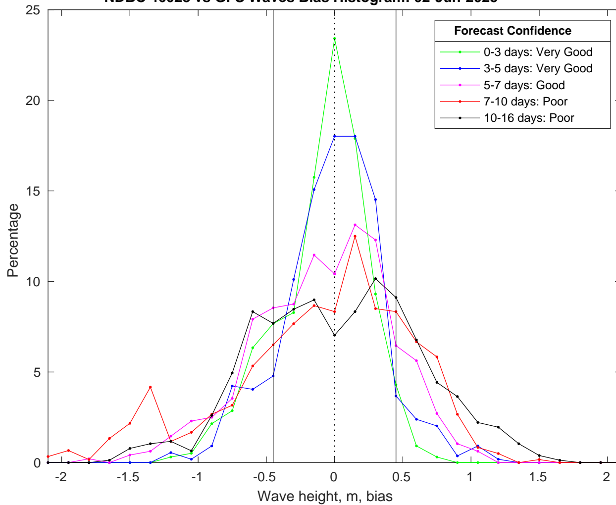
NDBC 46028 vs GFS Waves Bias Histogram: 02-Jun-2025
