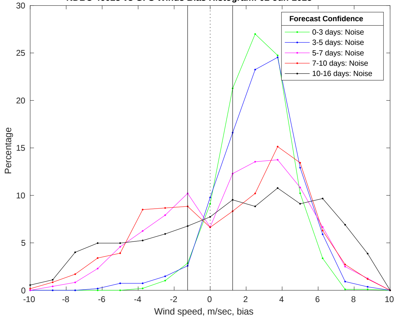
NDBC 46028 vs GFS Winds Bias Histogram: 02-Jun-2025
