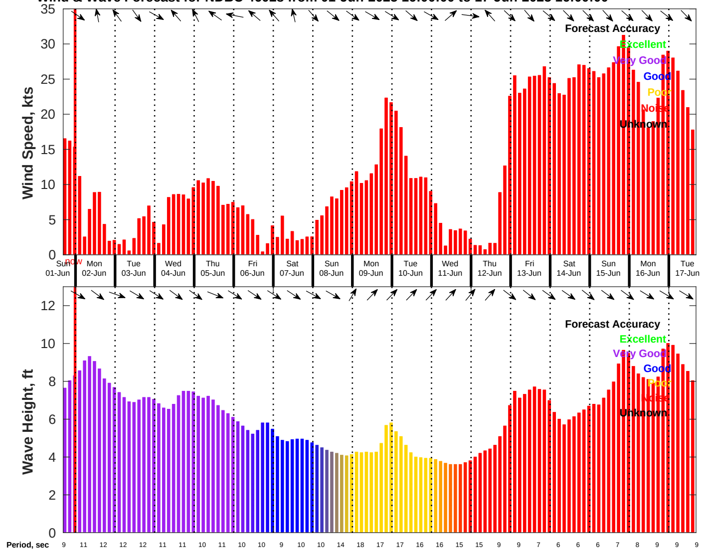
Wind & Wave Forecast for NDBC 46028 from 01-Jun-2025 16:00:00 to 17-Jun-2025 16:00:00
