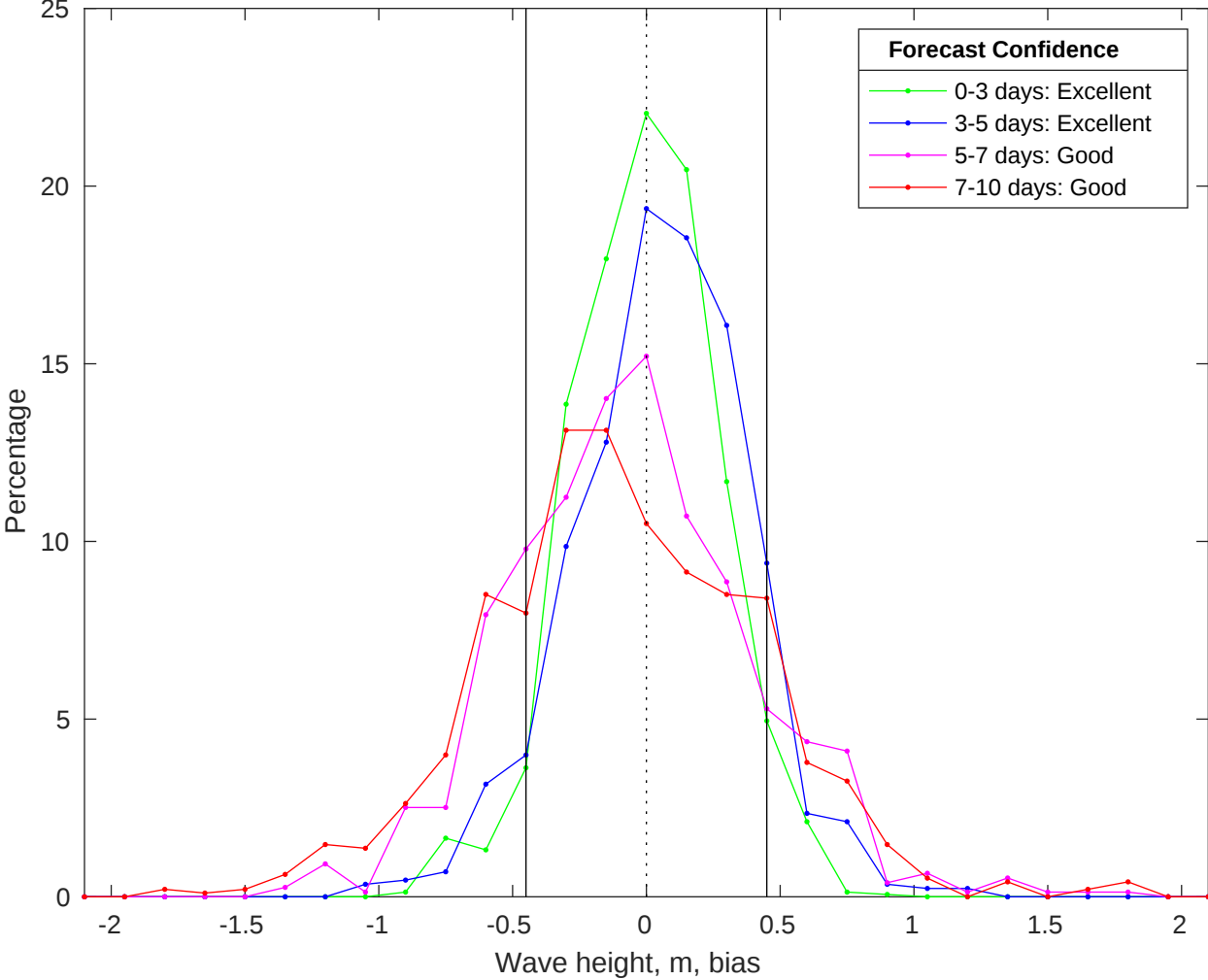
NDBC 46054 vs CMEMS Waves Bias Histogram: 02-Jun-2025
