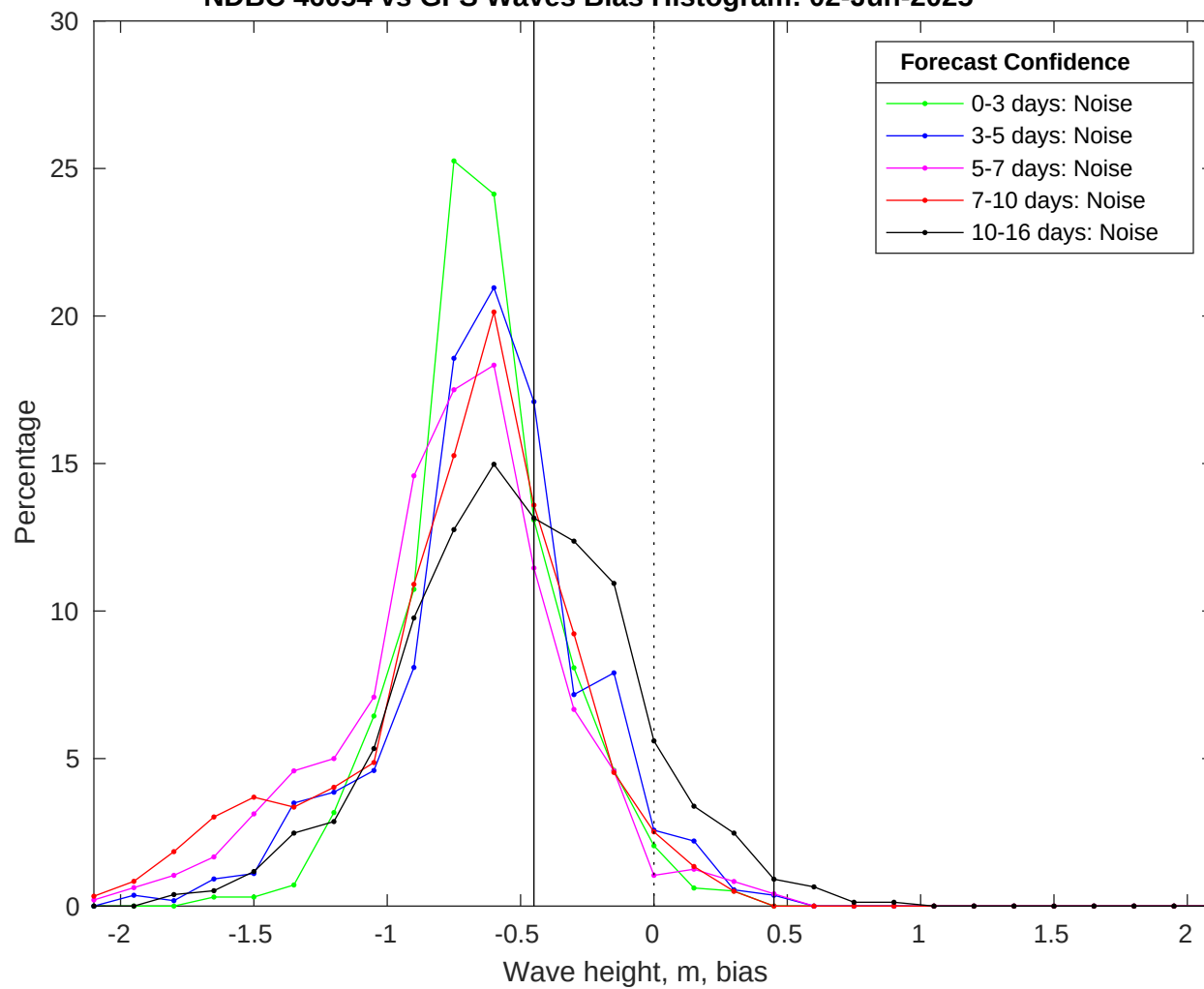
NDBC 46054 vs GFS Waves Bias Histogram: 02-Jun-2025
