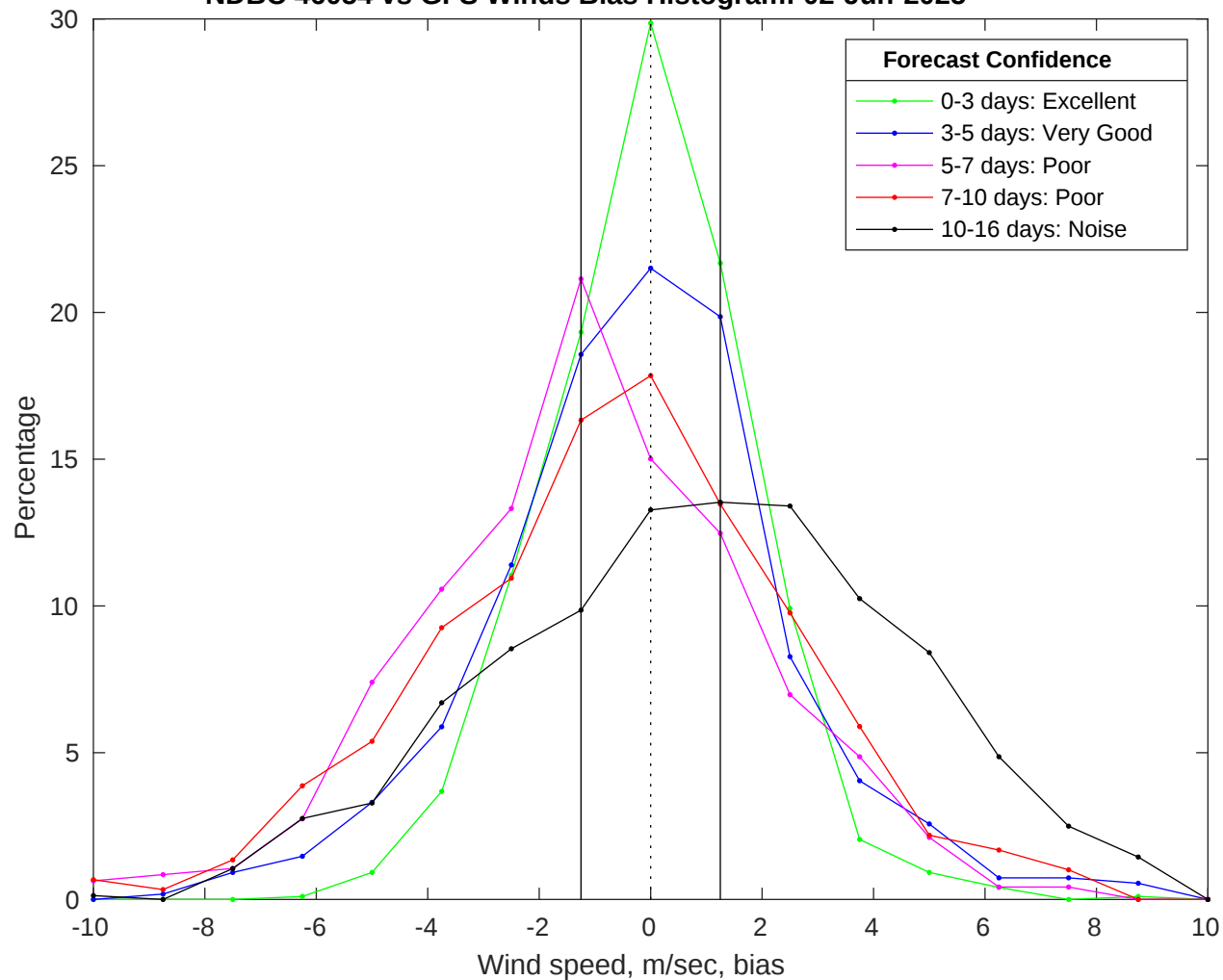
NDBC 46054 vs GFS Winds Bias Histogram: 02-Jun-2025
