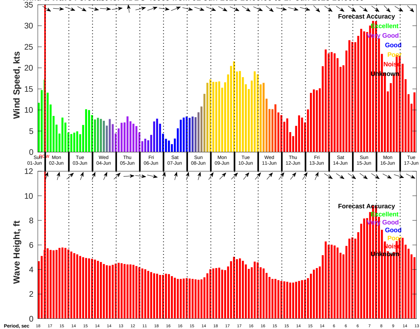
Wind & Wave Forecast for NDBC 46069 from 01-Jun-2025 16:00:00 to 17-Jun-2025 16:00:00
