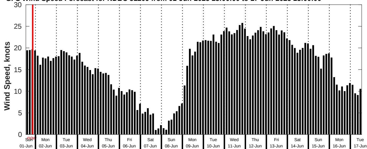
GFS Wind Speed Forecast for NDBC 51209 from 01-Jun-2025 13:00:00 to 17-Jun-2025 13:00:00
