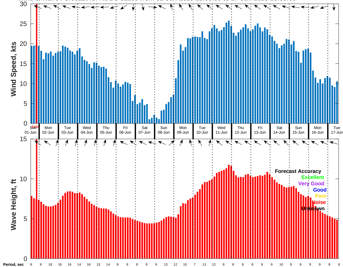
Wind & Wave Forecast for NDBC 51209 from 01-Jun-2025 13:00:00 to 17-Jun-2025 13:00:00
