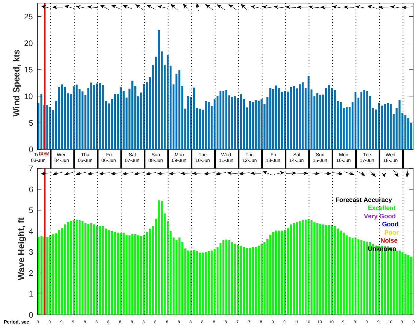
Wind & Wave Forecast for NDBC 52211 from 02-Jun-2025 10:00:00 to 18-Jun-2025 10:00:00
