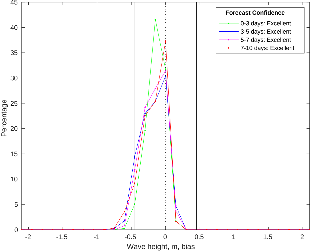
NDBC 52212 vs CMEMS Waves Bias Histogram: 02-Jun-2025
