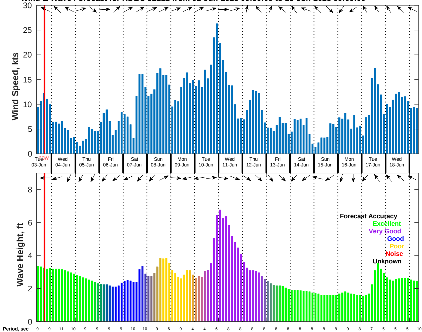
Wind & Wave Forecast for NDBC 52212 from 02-Jun-2025 09:00:00 to 18-Jun-2025 09:00:00
