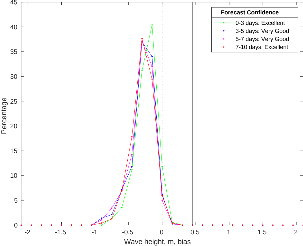
NDBC 52213 vs CMEMS Waves Bias Histogram: 02-Jun-2025
