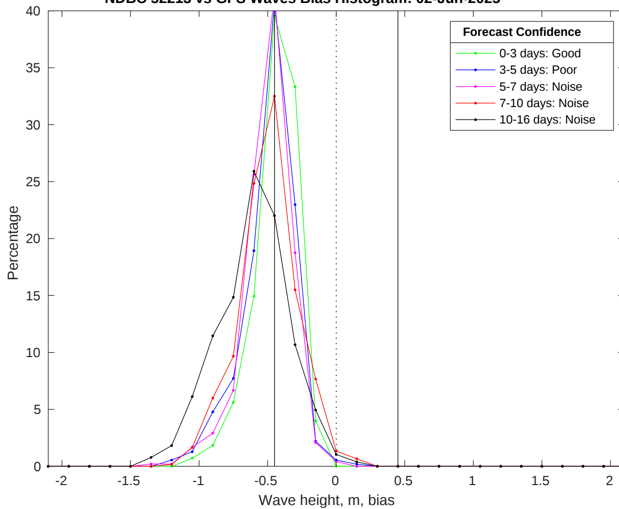
NDBC 52213 vs GFS Waves Bias Histogram: 02-Jun-2025
