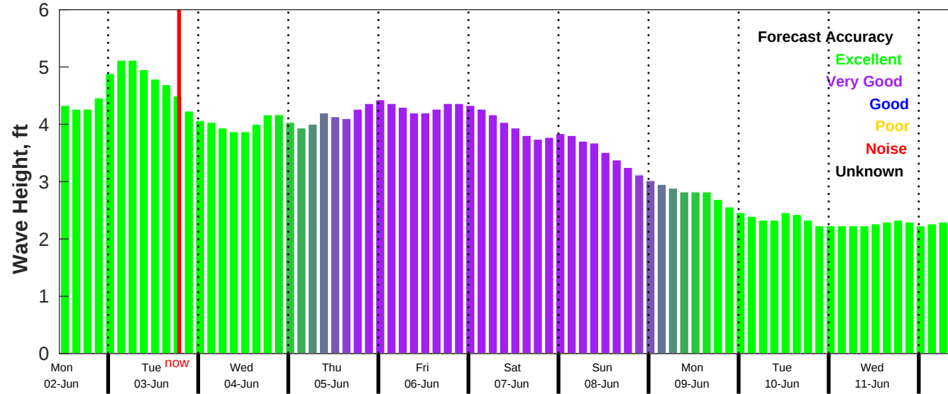
CMEMS Wave Forecast for NDBC 52213 from 01-Jun-2025 11:00:00 to 11-Jun-2025 11:00:00
