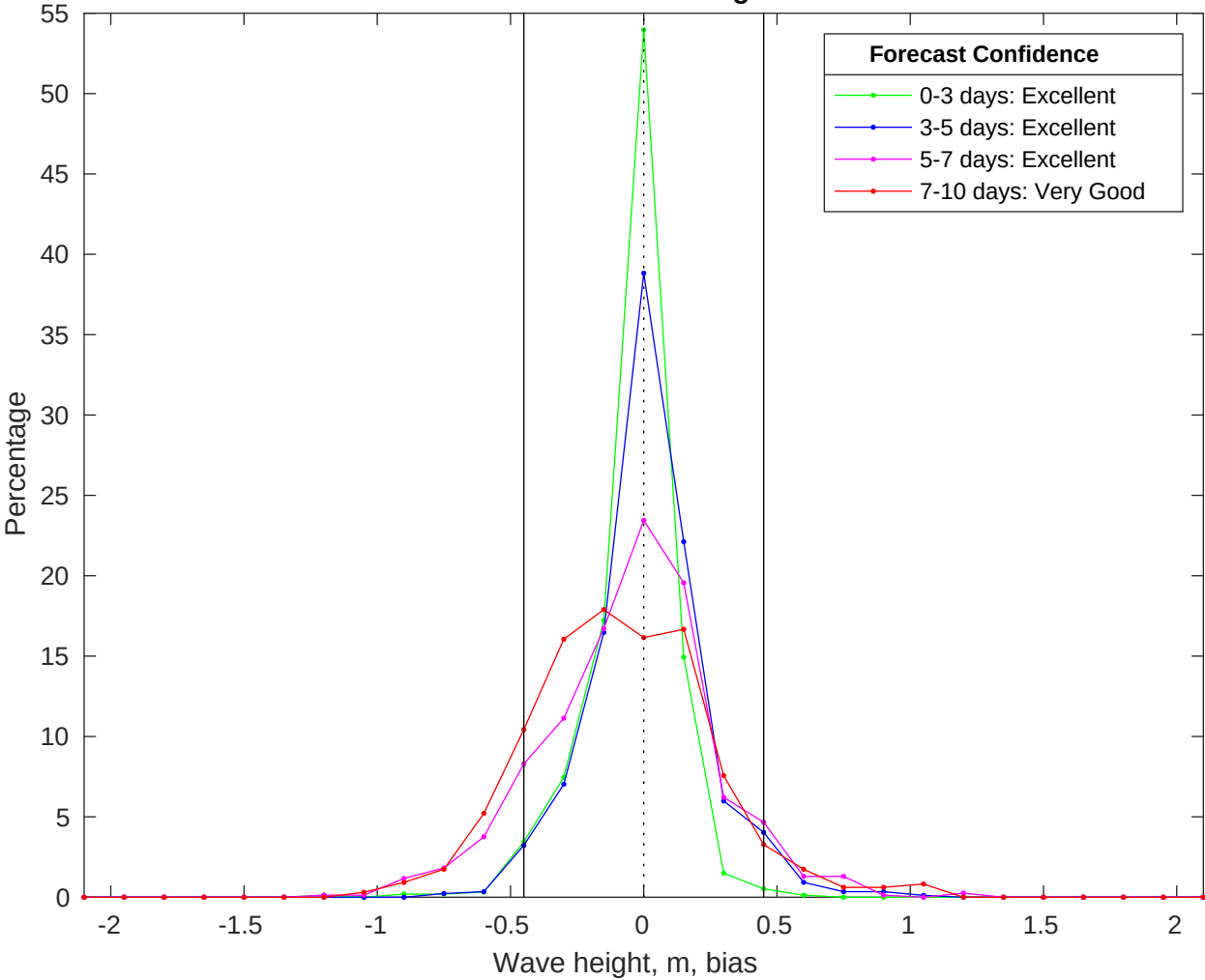
NDBC 41004 vs CMEMS Waves Bias Histogram: 03-Jun-2025
