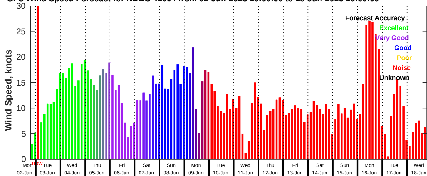
GFS Wind Speed Forecast for NDBC 41004 from 02-Jun-2025 19:00:00 to 18-Jun-2025 19:00:00
