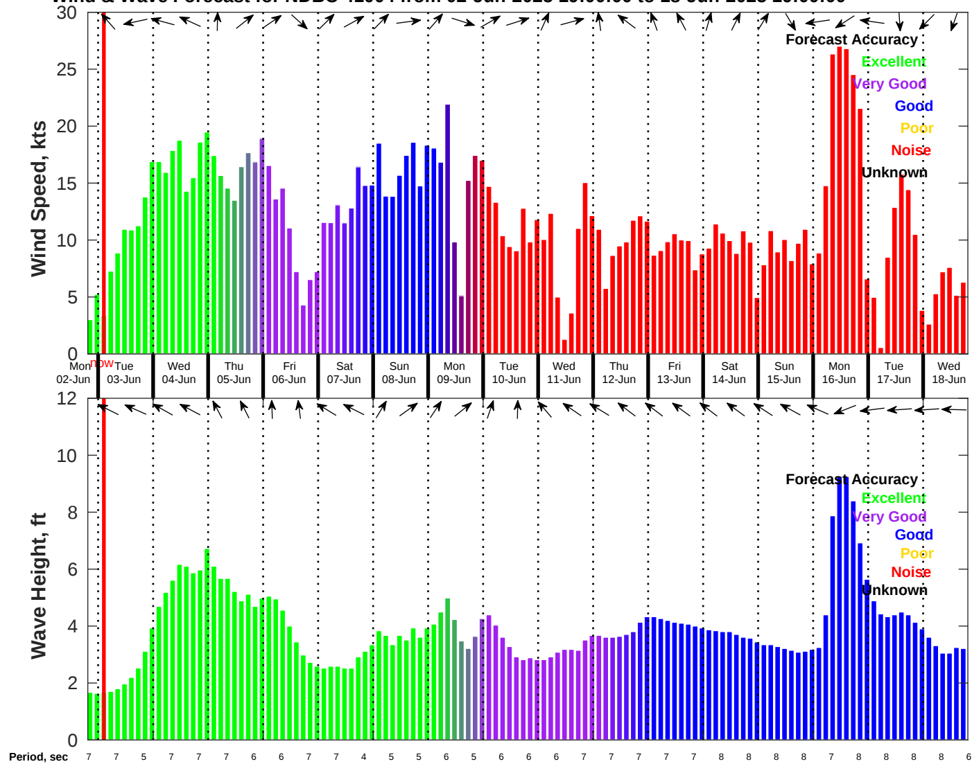
Wind & Wave Forecast for NDBC 41004 from 02-Jun-2025 19:00:00 to 18-Jun-2025 19:00:00
