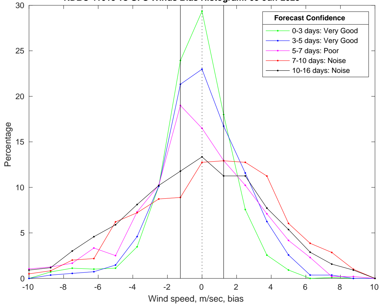
NDBC 41013 vs GFS Winds Bias Histogram: 03-Jun-2025
