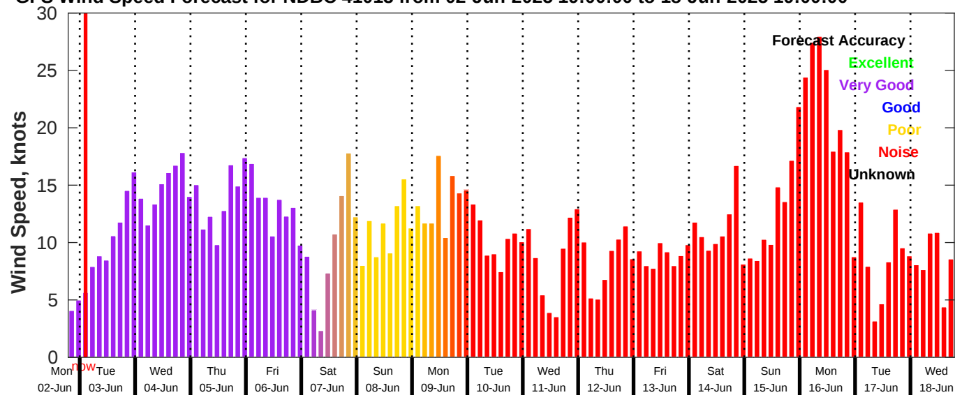
GFS Wind Speed Forecast for NDBC 41013 from 02-Jun-2025 19:00:00 to 18-Jun-2025 19:00:00
