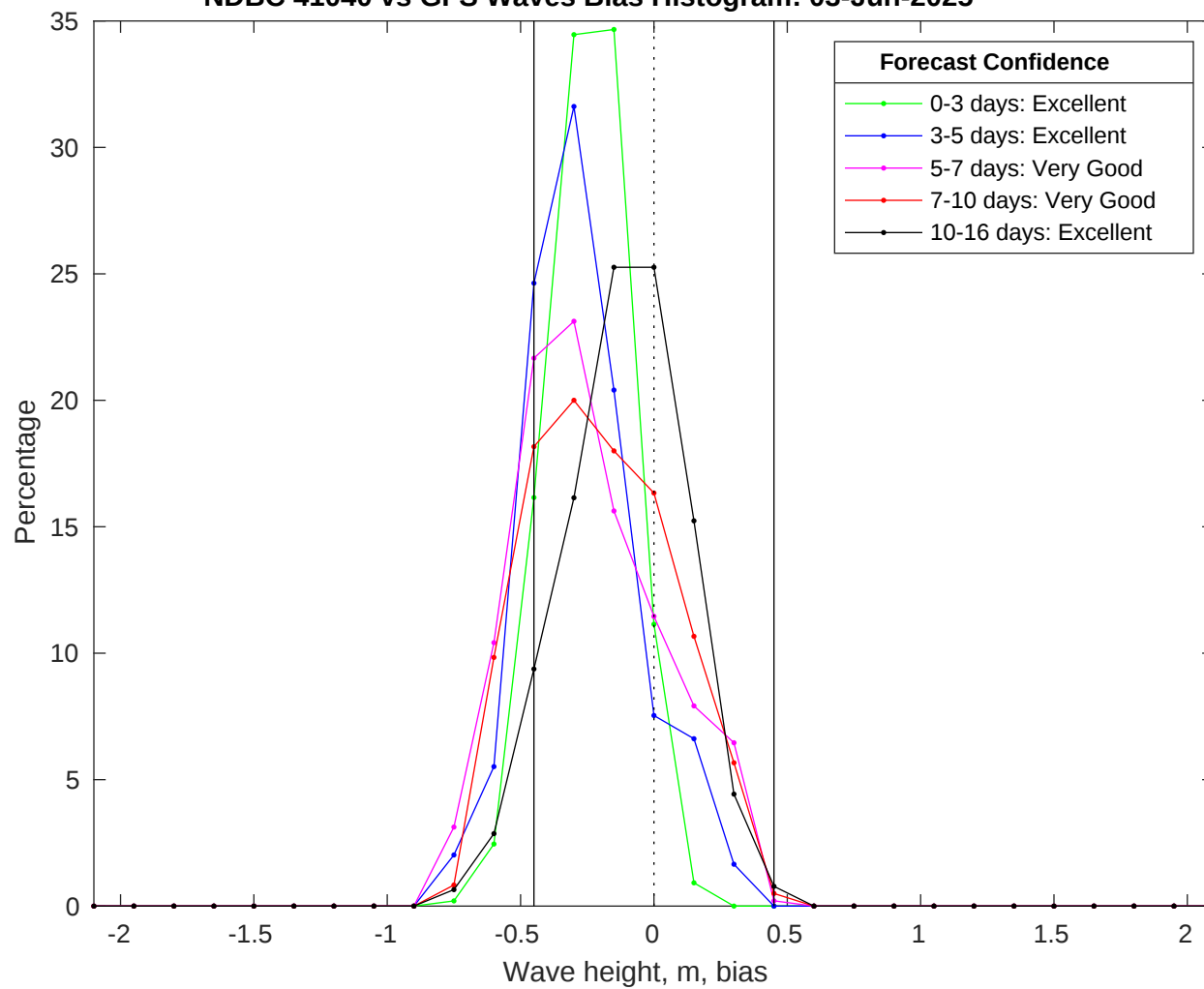
NDBC 41040 vs GFS Waves Bias Histogram: 03-Jun-2025
