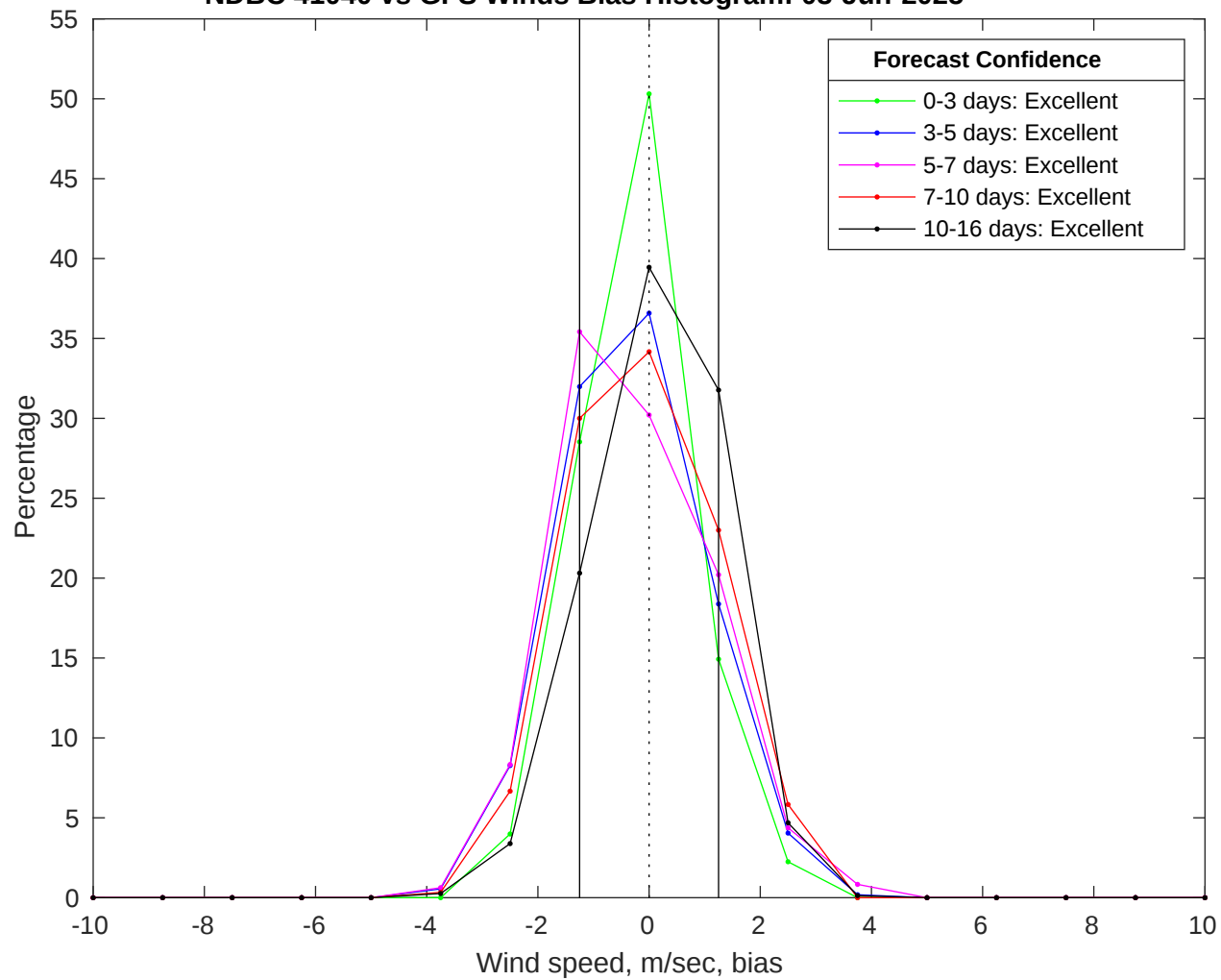
NDBC 41040 vs GFS Winds Bias Histogram: 03-Jun-2025
