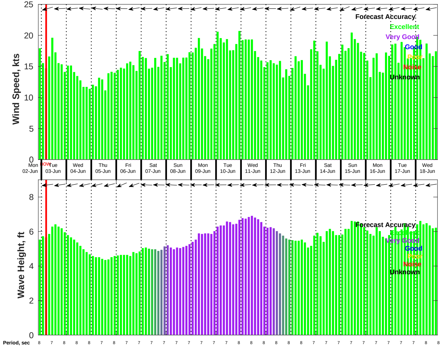
Wind & Wave Forecast for NDBC 41040 from 02-Jun-2025 21:00:00 to 18-Jun-2025 21:00:00
