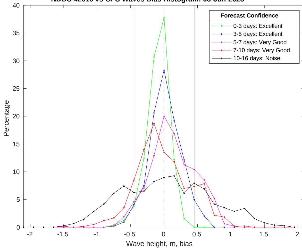
NDBC 42019 vs GFS Waves Bias Histogram: 03-Jun-2025
