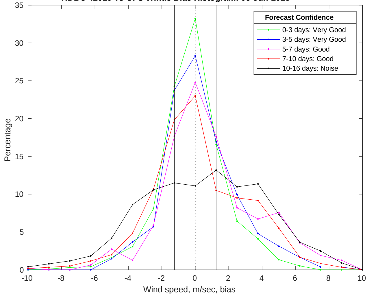
NDBC 42019 vs GFS Winds Bias Histogram: 03-Jun-2025
