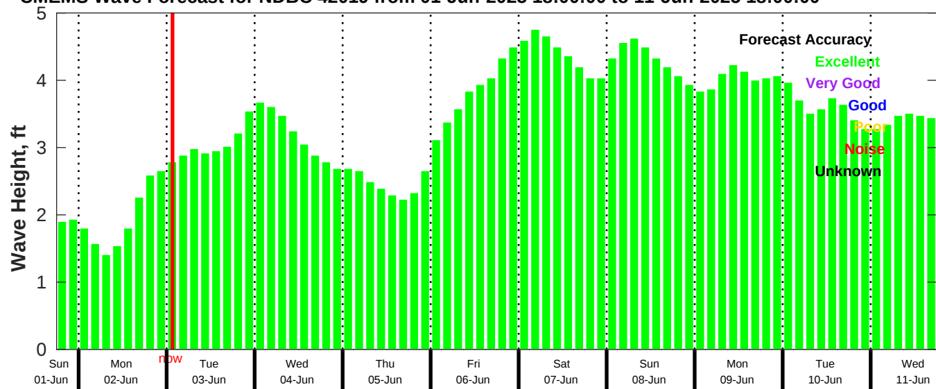
CMEMS Wave Forecast for NDBC 42019 from 01-Jun-2025 18:00:00 to 11-Jun-2025 18:00:00
