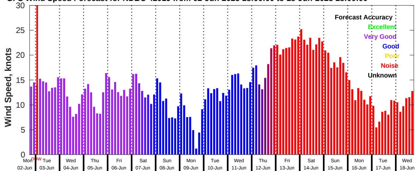
GFS Wind Speed Forecast for NDBC 42019 from 02-Jun-2025 18:00:00 to 18-Jun-2025 18:00:00
