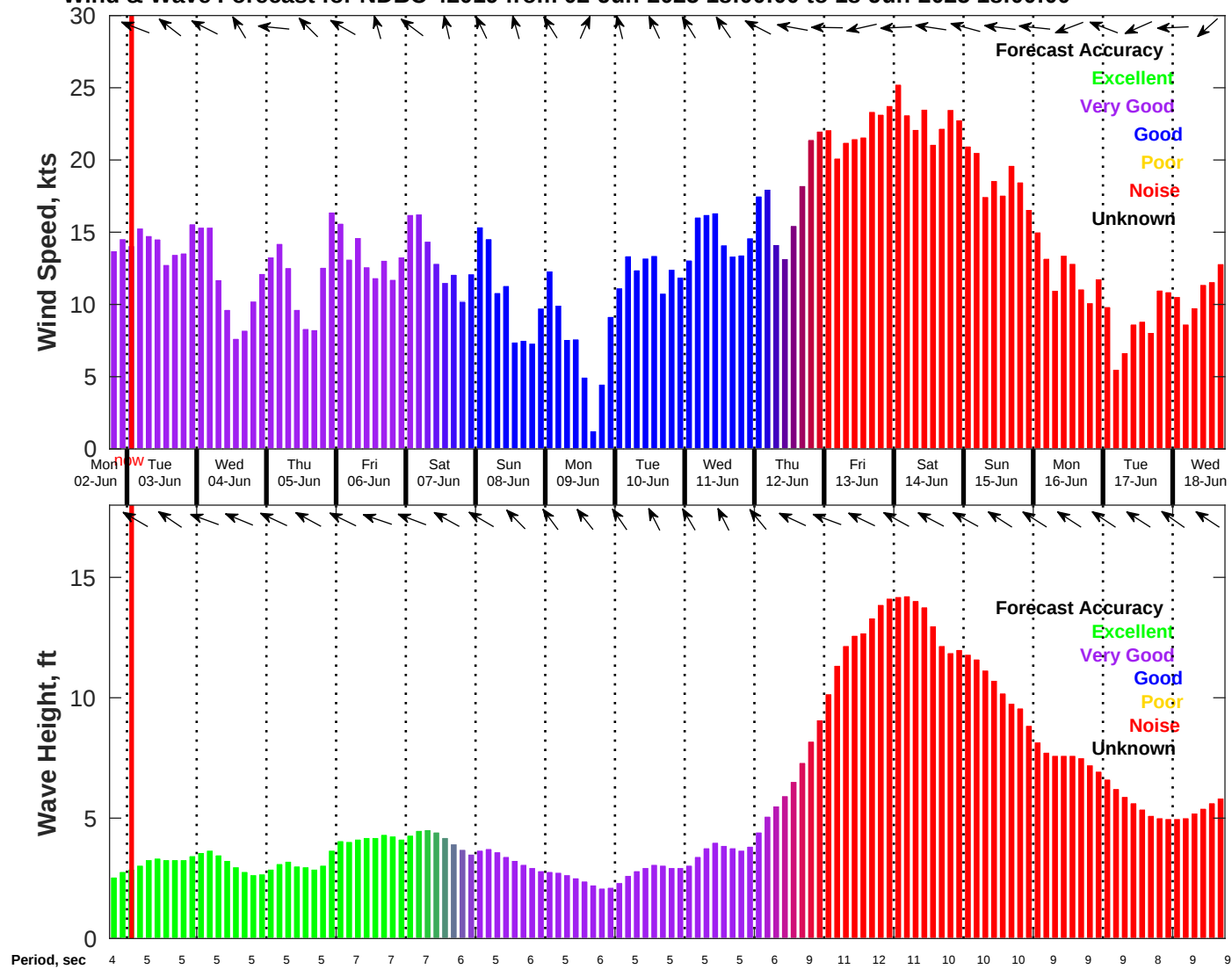
Wind & Wave Forecast for NDBC 42019 from 02-Jun-2025 18:00:00 to 18-Jun-2025 18:00:00
