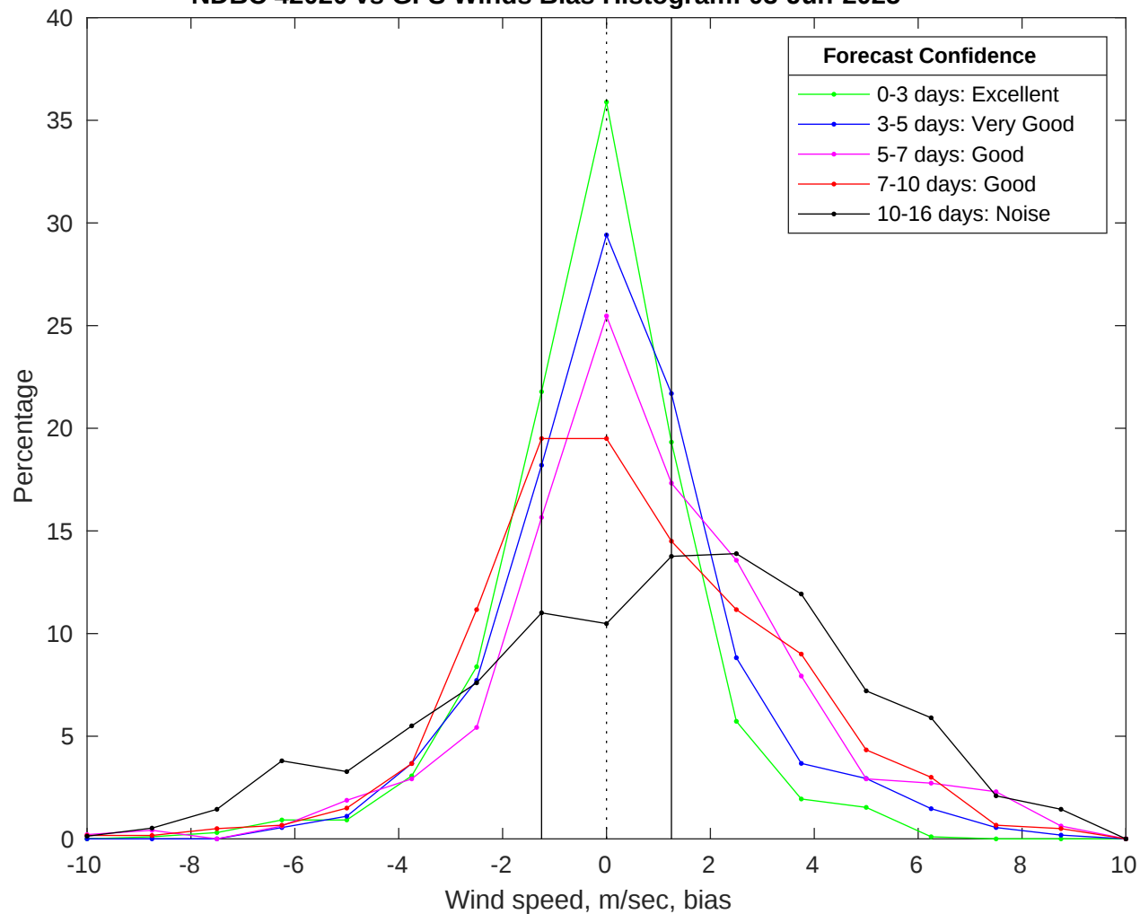
NDBC 42020 vs GFS Winds Bias Histogram: 03-Jun-2025
