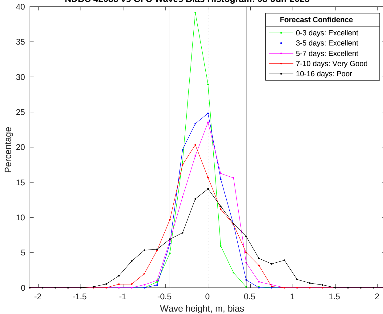
NDBC 42035 vs GFS Waves Bias Histogram: 03-Jun-2025
