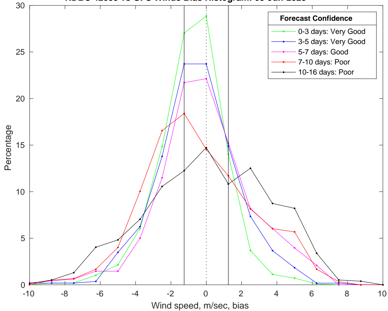
NDBC 42035 vs GFS Winds Bias Histogram: 03-Jun-2025
