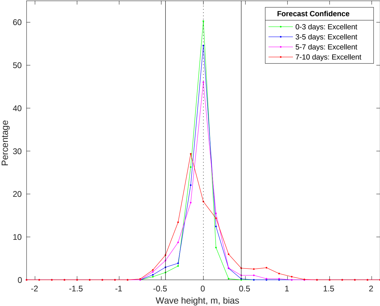
NDBC 42036 vs CMEMS Waves Bias Histogram: 03-Jun-2025
