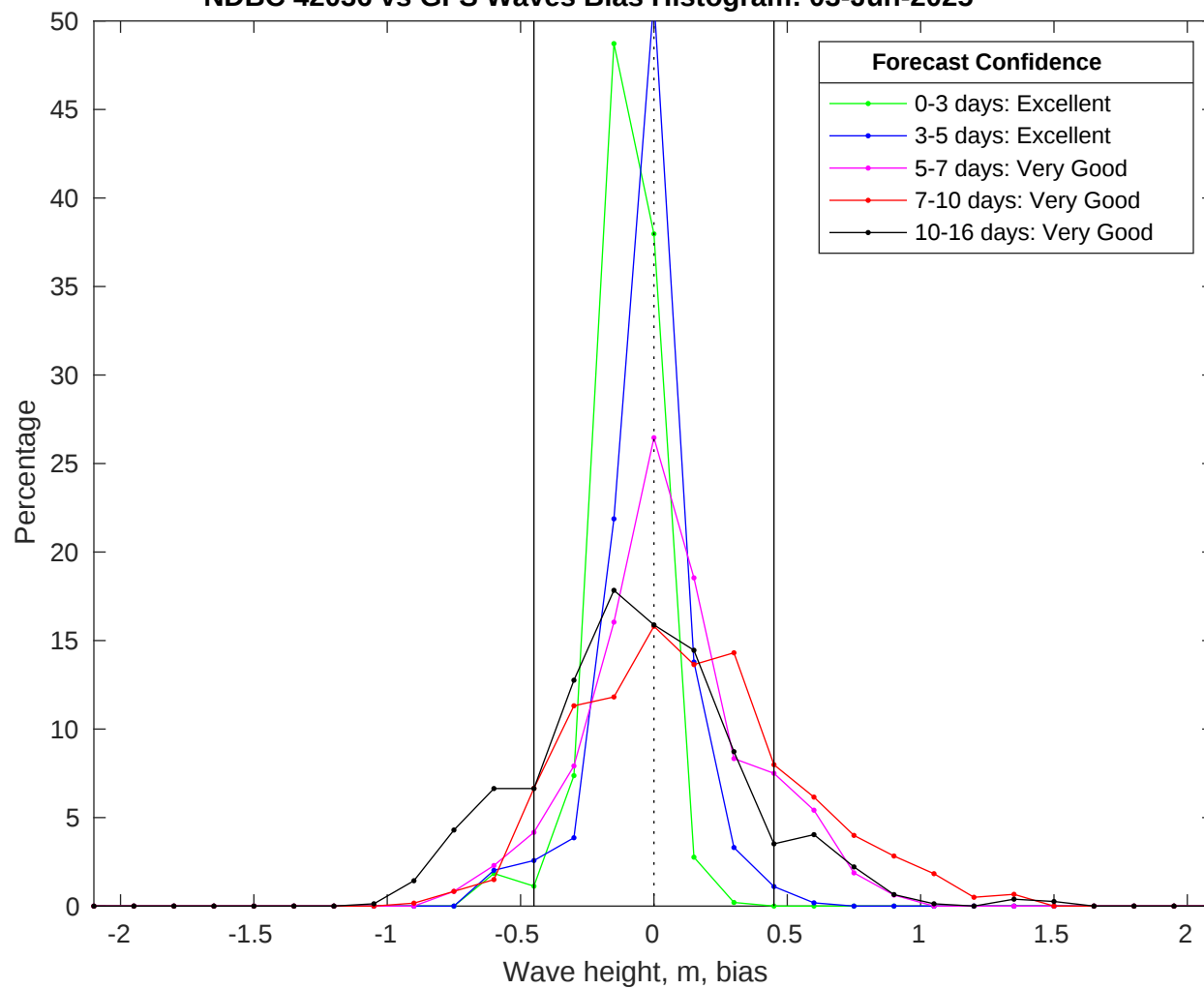
NDBC 42036 vs GFS Waves Bias Histogram: 03-Jun-2025
