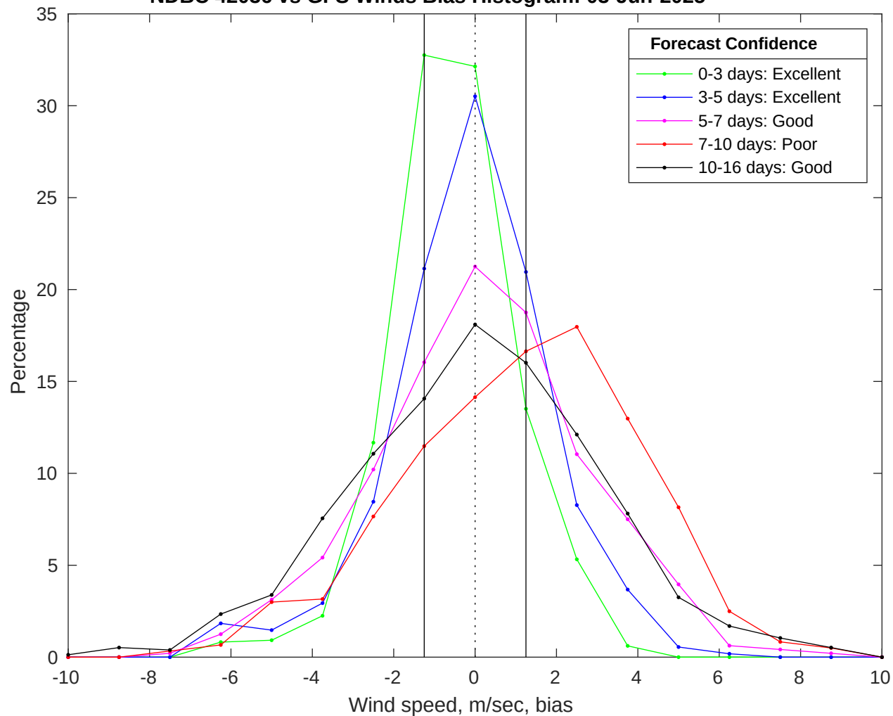
NDBC 42036 vs GFS Winds Bias Histogram: 03-Jun-2025
