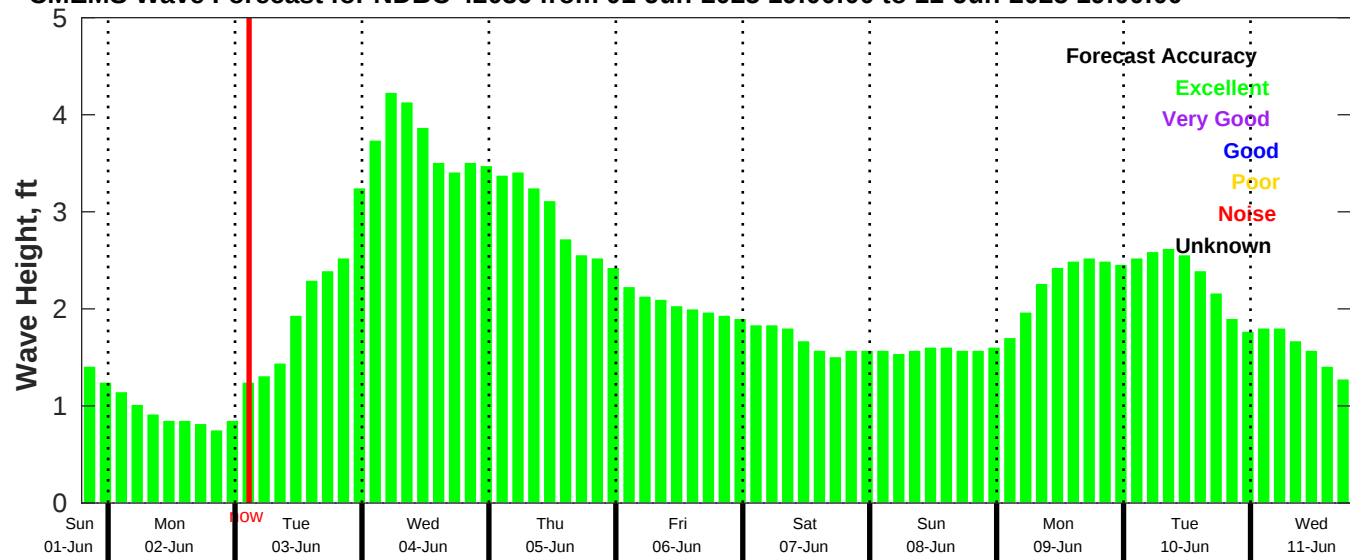
CMEMS Wave Forecast for NDBC 42036 from 01-Jun-2025 19:00:00 to 11-Jun-2025 19:00:00
