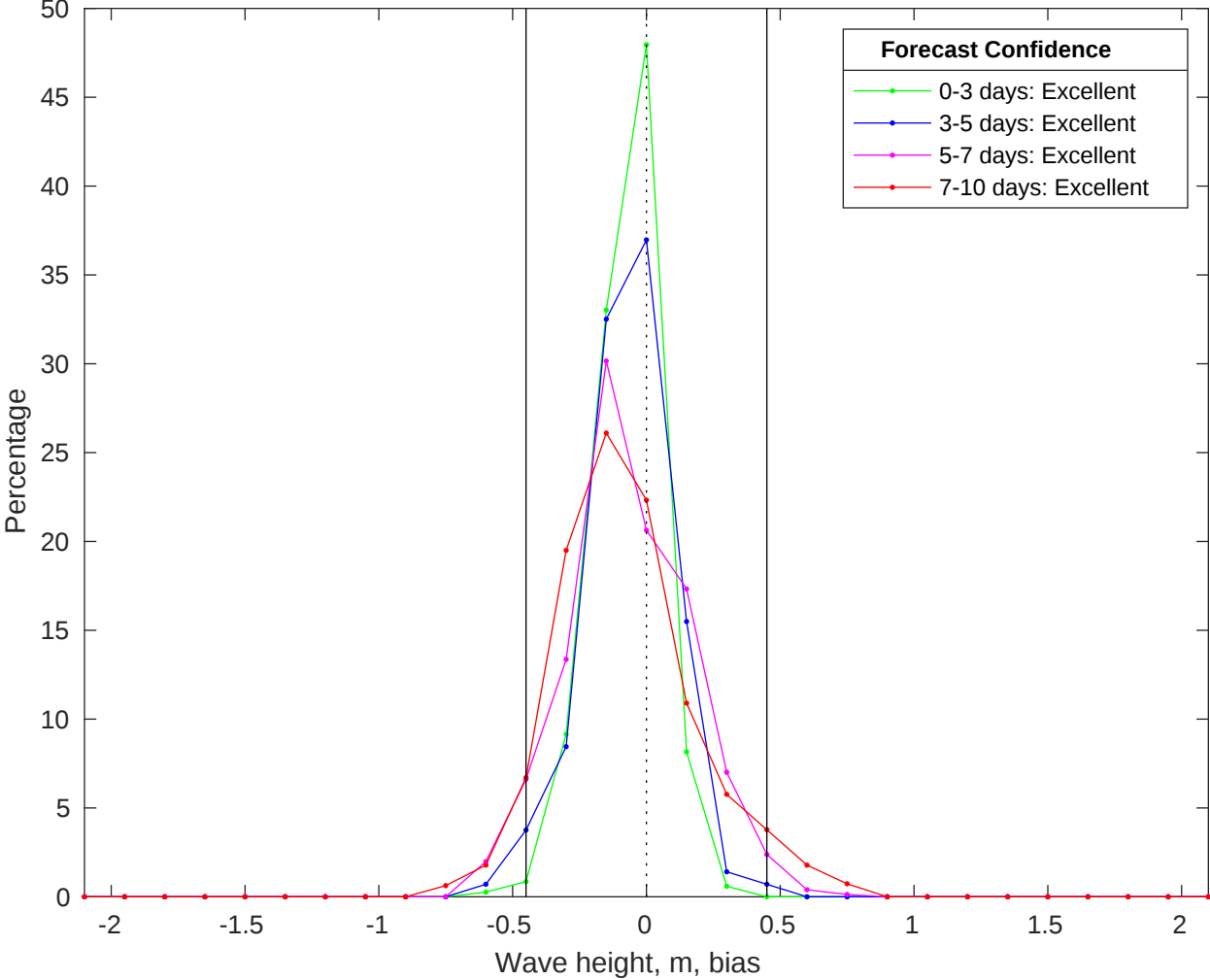
NDBC 42040 vs CMEMS Waves Bias Histogram: 03-Jun-2025
