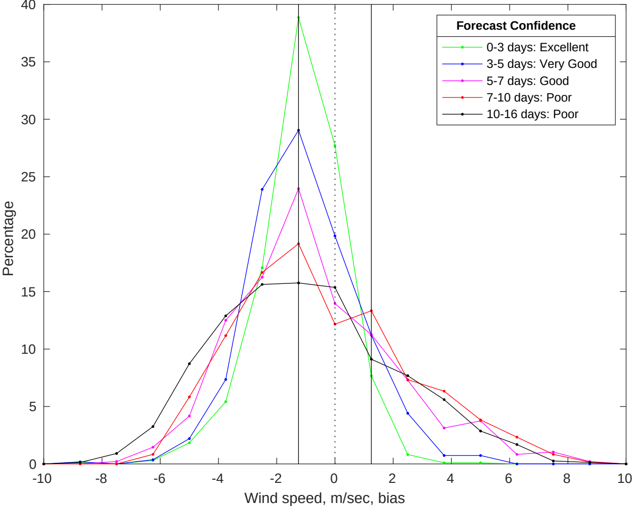
NDBC 42040 vs GFS Winds Bias Histogram: 03-Jun-2025
