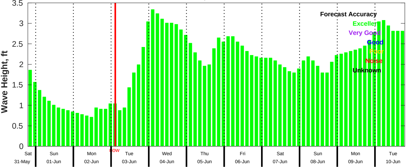
CMEMS Wave Forecast for NDBC 42040 from 31-May-2025 19:00:00 to 10-Jun-2025 19:00:00
