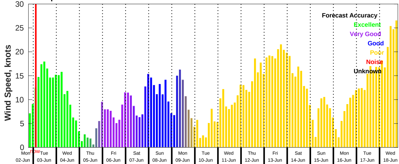
GFS Wind Speed Forecast for NDBC 42040 from 02-Jun-2025 19:00:00 to 18-Jun-2025 19:00:00
