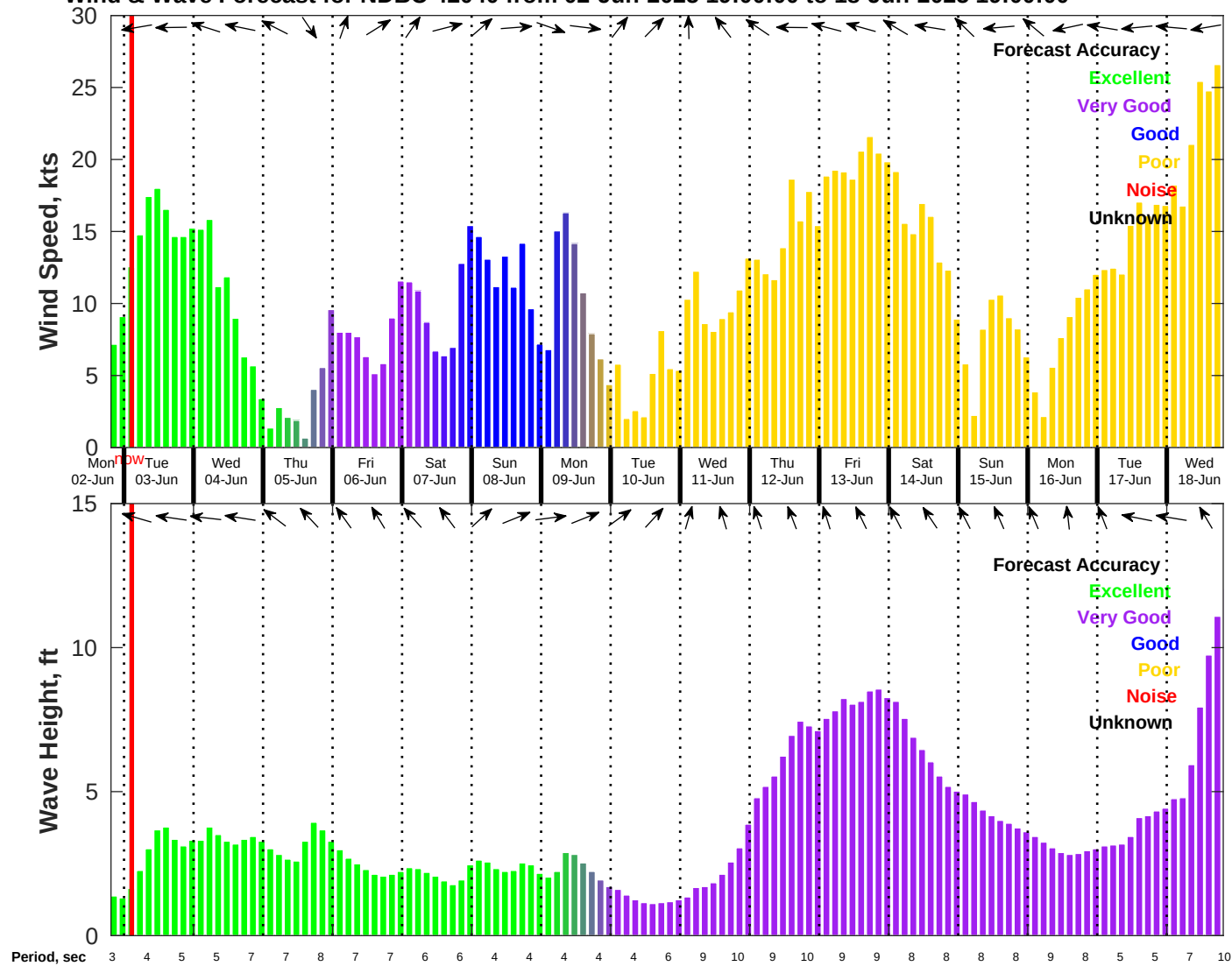
Wind & Wave Forecast for NDBC 42040 from 02-Jun-2025 19:00:00 to 18-Jun-2025 19:00:00
