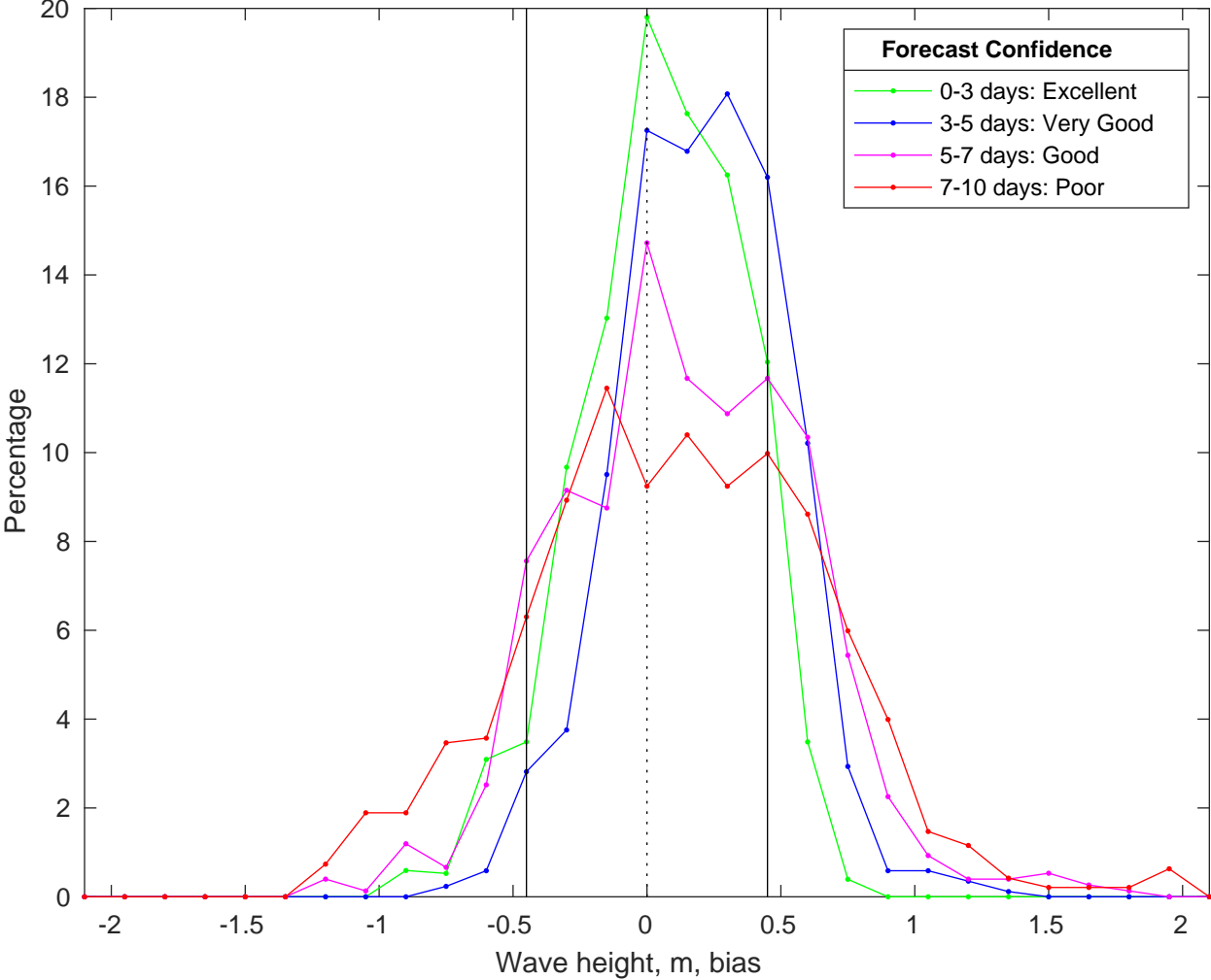
NDBC 46011 vs CMEMS Waves Bias Histogram: 03-Jun-2025
