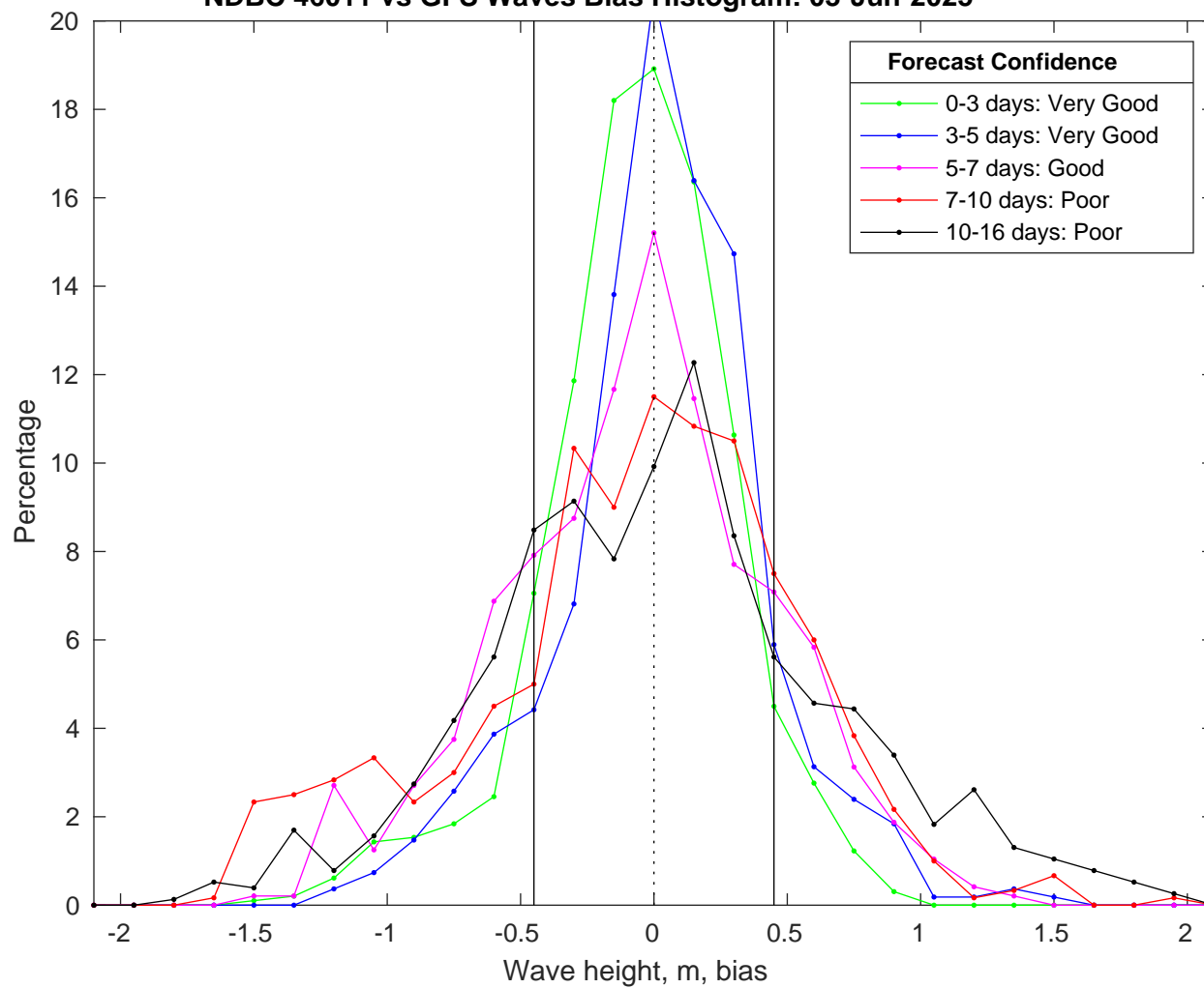
NDBC 46011 vs GFS Waves Bias Histogram: 03-Jun-2025
