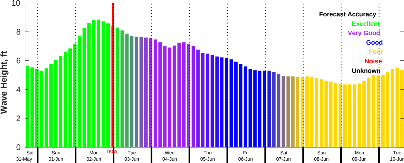
CMEMS Wave Forecast for NDBC 46011 from 31-May-2025 16:00:00 to 10-Jun-2025 16:00:00
