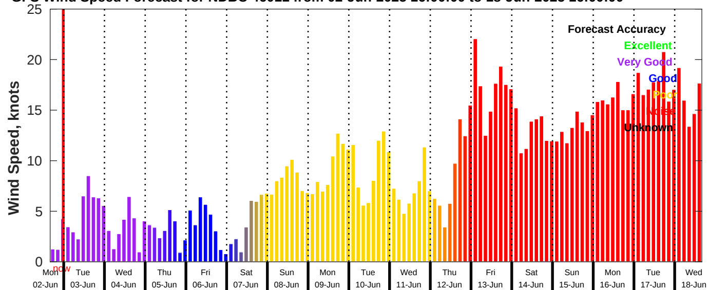
GFS Wind Speed Forecast for NDBC 46011 from 02-Jun-2025 16:00:00 to 18-Jun-2025 16:00:00
