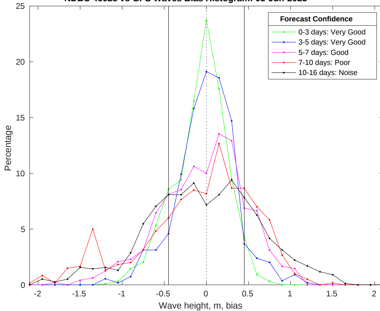
NDBC 46028 vs GFS Waves Bias Histogram: 03-Jun-2025
