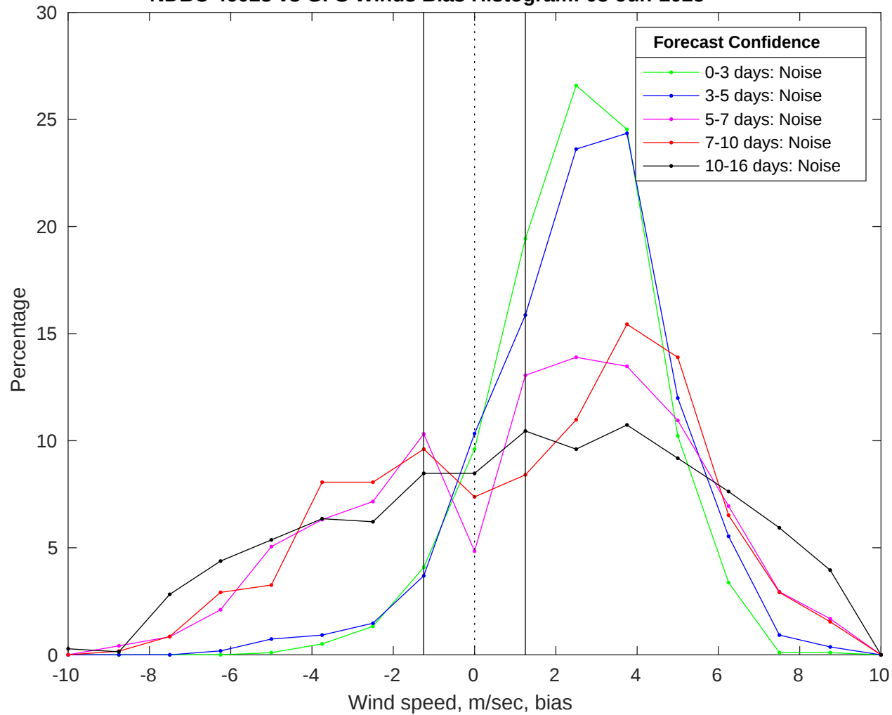
NDBC 46028 vs GFS Winds Bias Histogram: 03-Jun-2025
