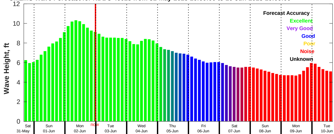
CMEMS Wave Forecast for NDBC 46028 from 31-May-2025 16:00:00 to 10-Jun-2025 16:00:00
