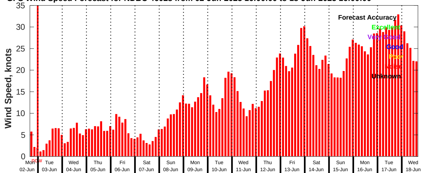
GFS Wind Speed Forecast for NDBC 46028 from 02-Jun-2025 16:00:00 to 18-Jun-2025 16:00:00
