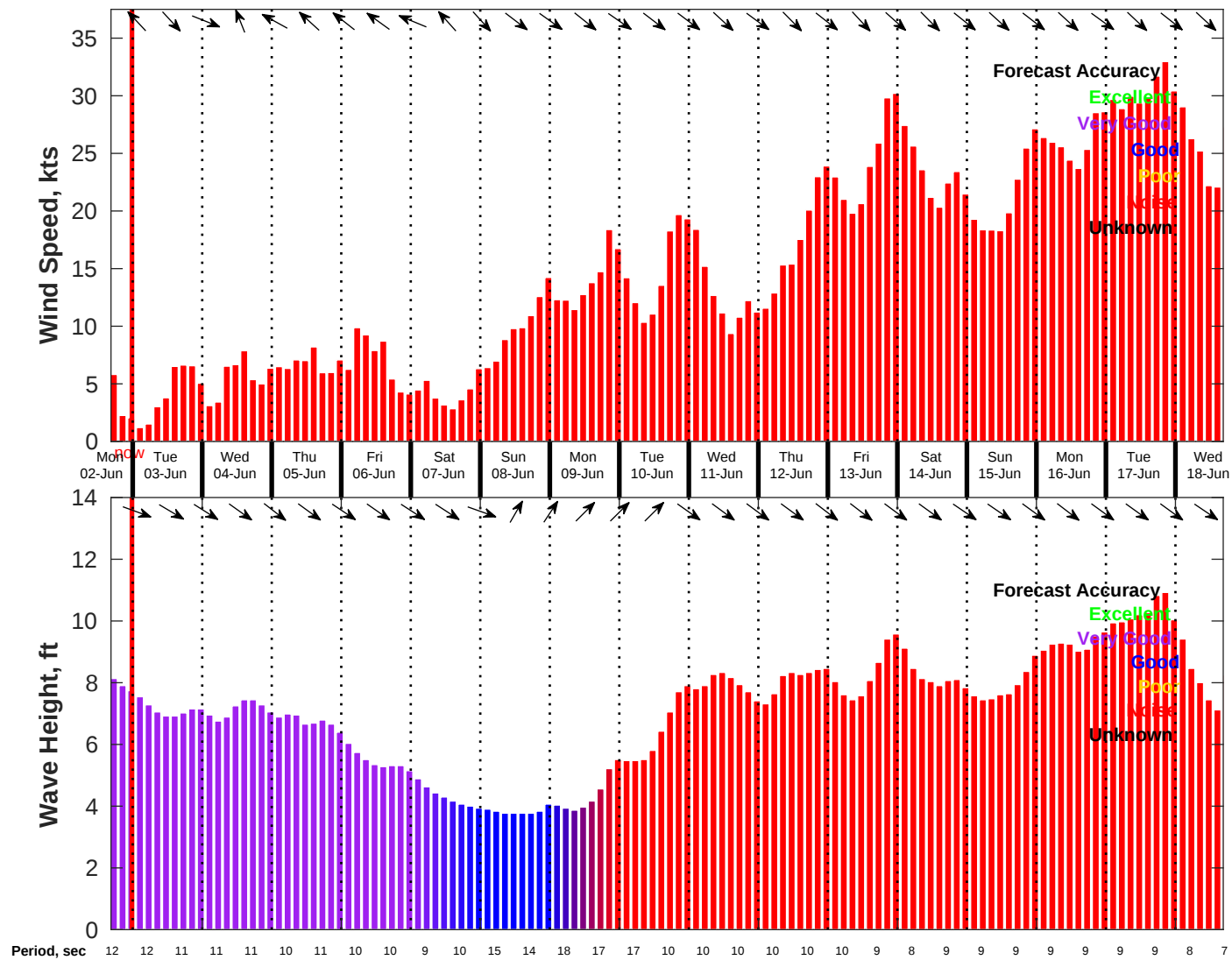
Wind & Wave Forecast for NDBC 46028 from 02-Jun-2025 16:00:00 to 18-Jun-2025 16:00:00
