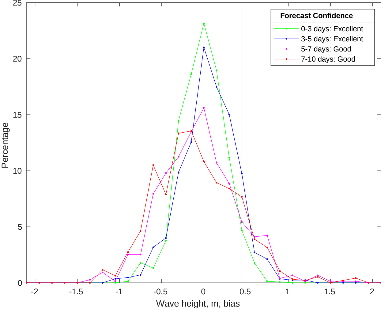
NDBC 46054 vs CMEMS Waves Bias Histogram: 03-Jun-2025
